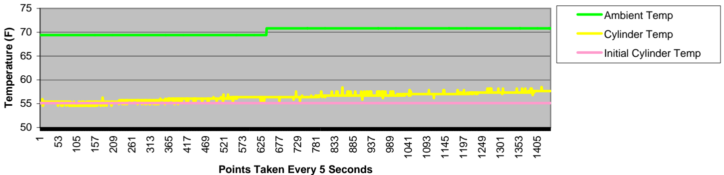
COMPRESSOR CYLINDER HYRDO TEST Temperature Chart
